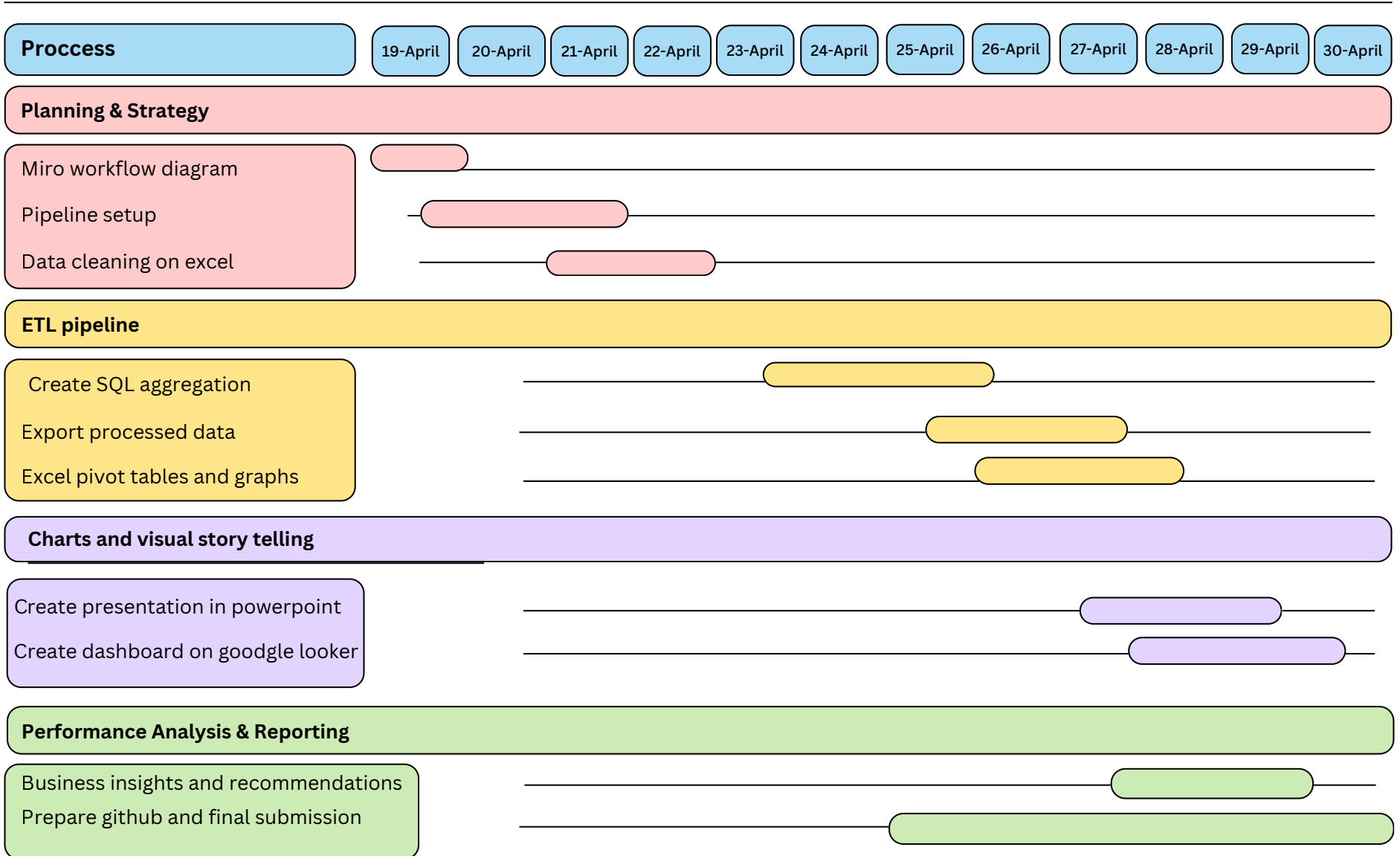
Gantt Chart
